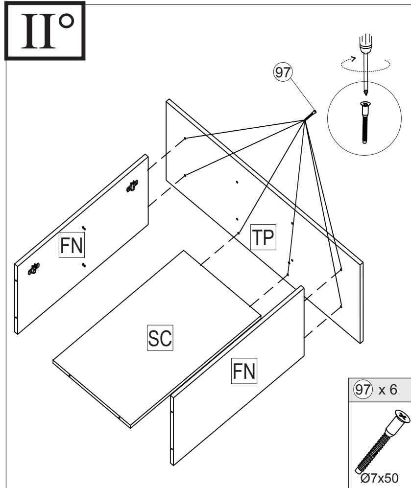
MOBILE DUBAI 100 1010x410x730
